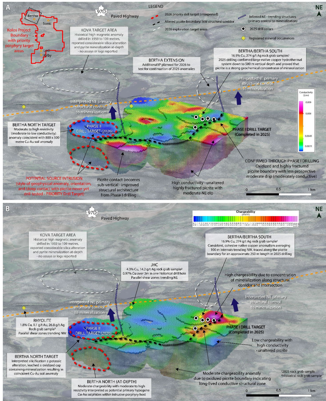
Figure 1. Inverted IP conductivity (A) and chargeability (B) showcasing picrite contact, registered mineral occurrences with select annotated rock grab samples, and priority exploration drill targets.
