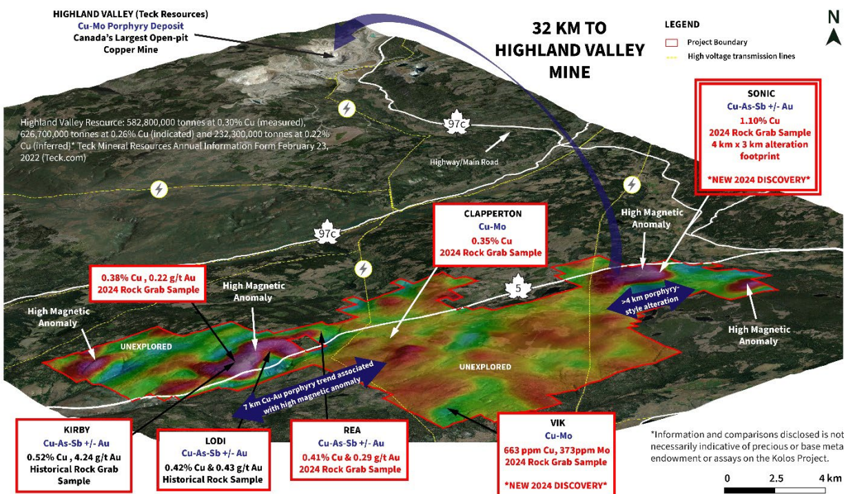
Figure 1. Kolos Project area overlying the vertical derivative of the residual magnetic intensity (RMI) geophysical survey with annotated exploration targets, 2024 rock grab sample outcrop locations, and additional unexplored high magnetic exploration targets.
