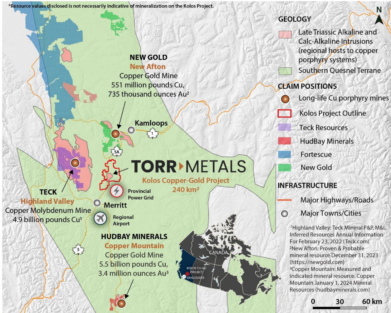
Figure 2. Kolos Project location within the prolific porphyry belt of the Quesnel Terrane in south-central British Columbia. Figure including locations of Late Triassic Alkaline and Calc-Alkaline intrusions modified from Mitchinson et al. 2024 2 .
